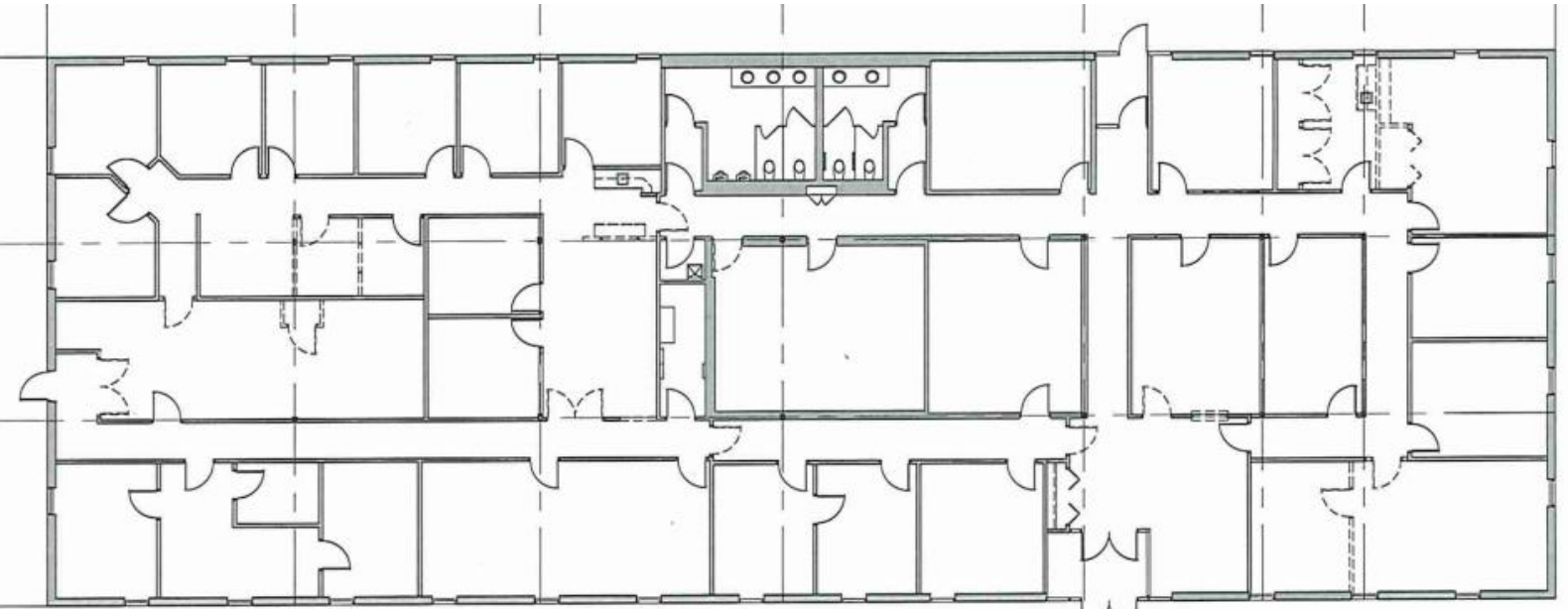
DEMOLITION FLOOR PLAN
