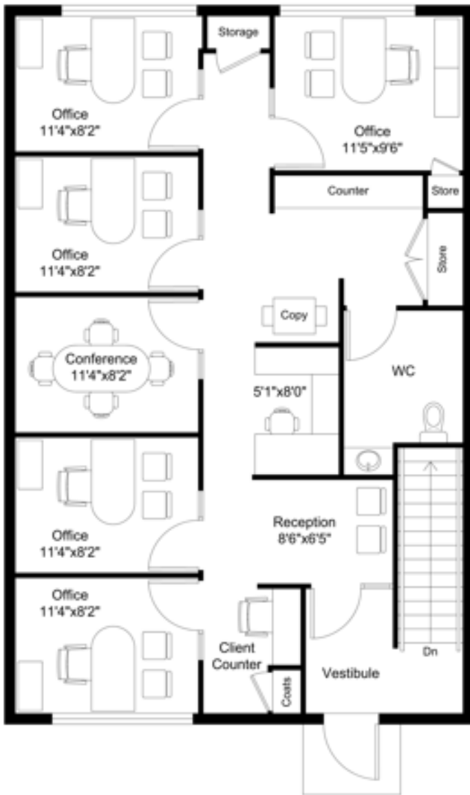
UPPER FLOOR
